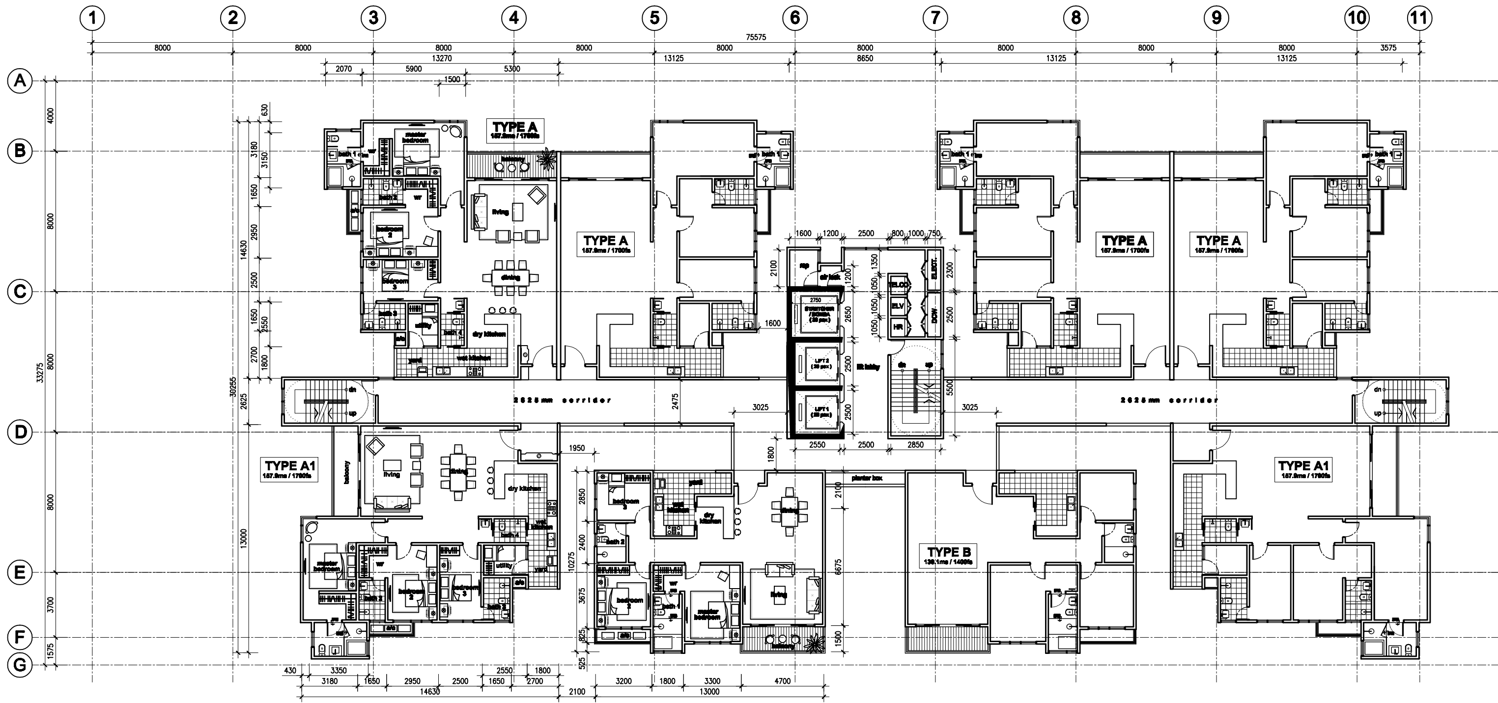
CONDO TYPICAL LAYOUT PLAN - 8 UNIT PER FLOOR
